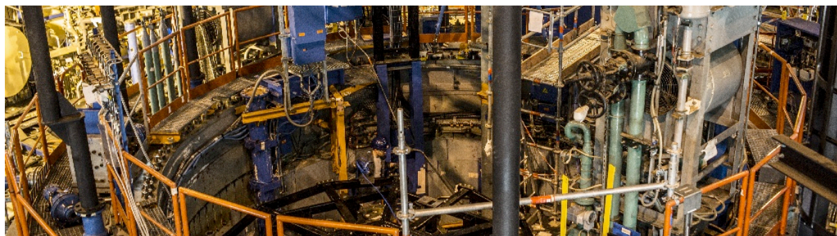
Figure 1: Creys Malville site under decommissioning (EDF-Sophie Brandstrom)
